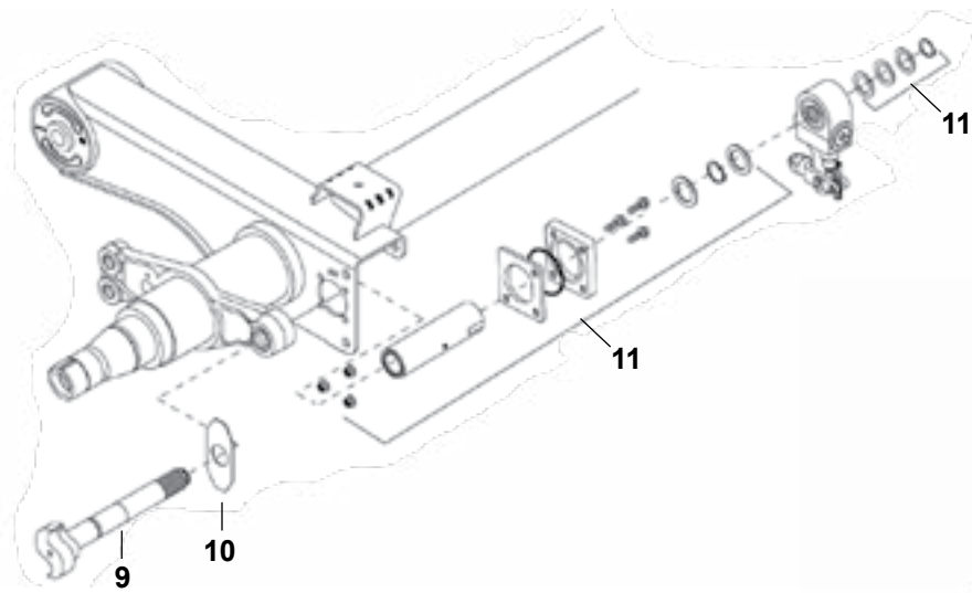
Camshaft, Bushings & Bracket Parts New Style, Enclosed Cam Tube
