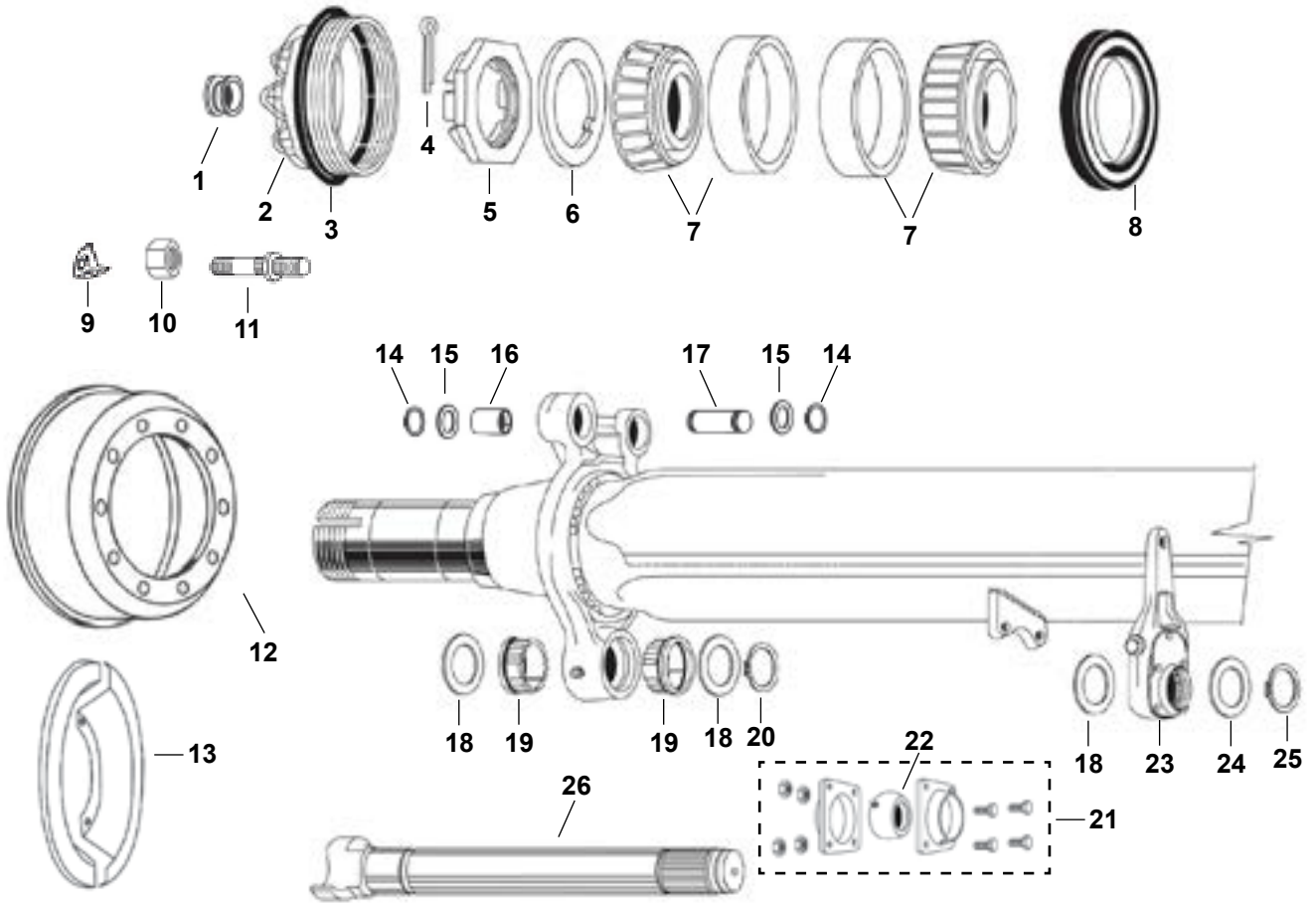
OLD STYLE "XEM" BRAKE
