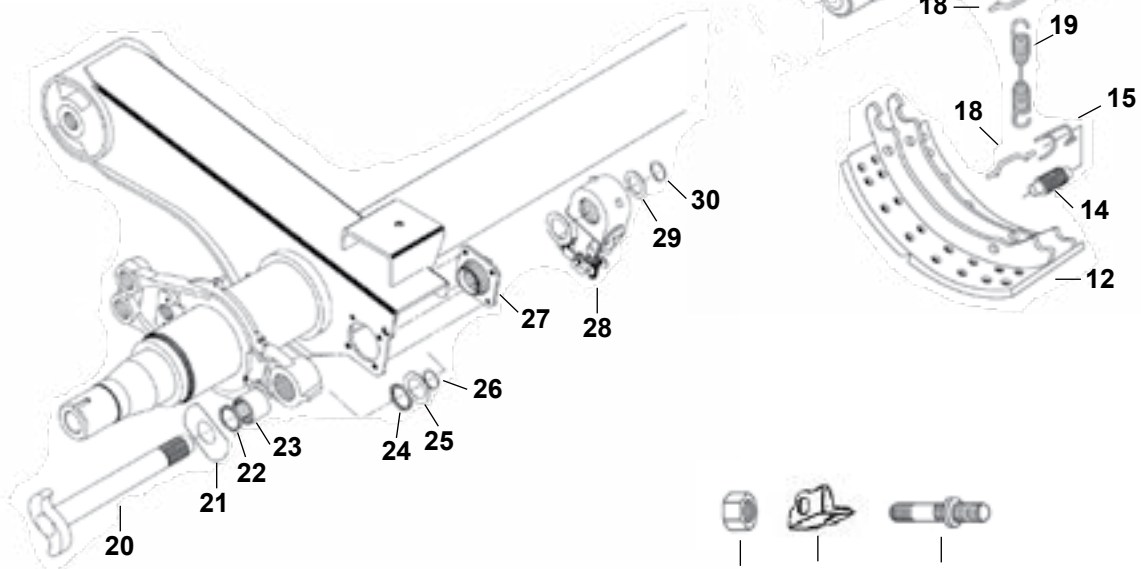
Camshaft, Bushings & Bracket Parts Old Style, Exposed Cam Tube
